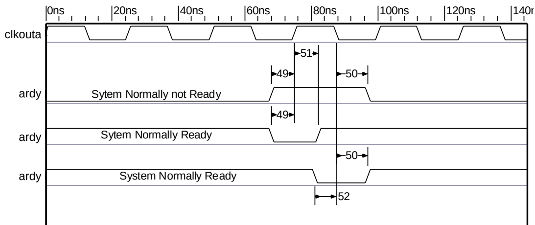
Figure 23. ardy—Asynchronous Ready
