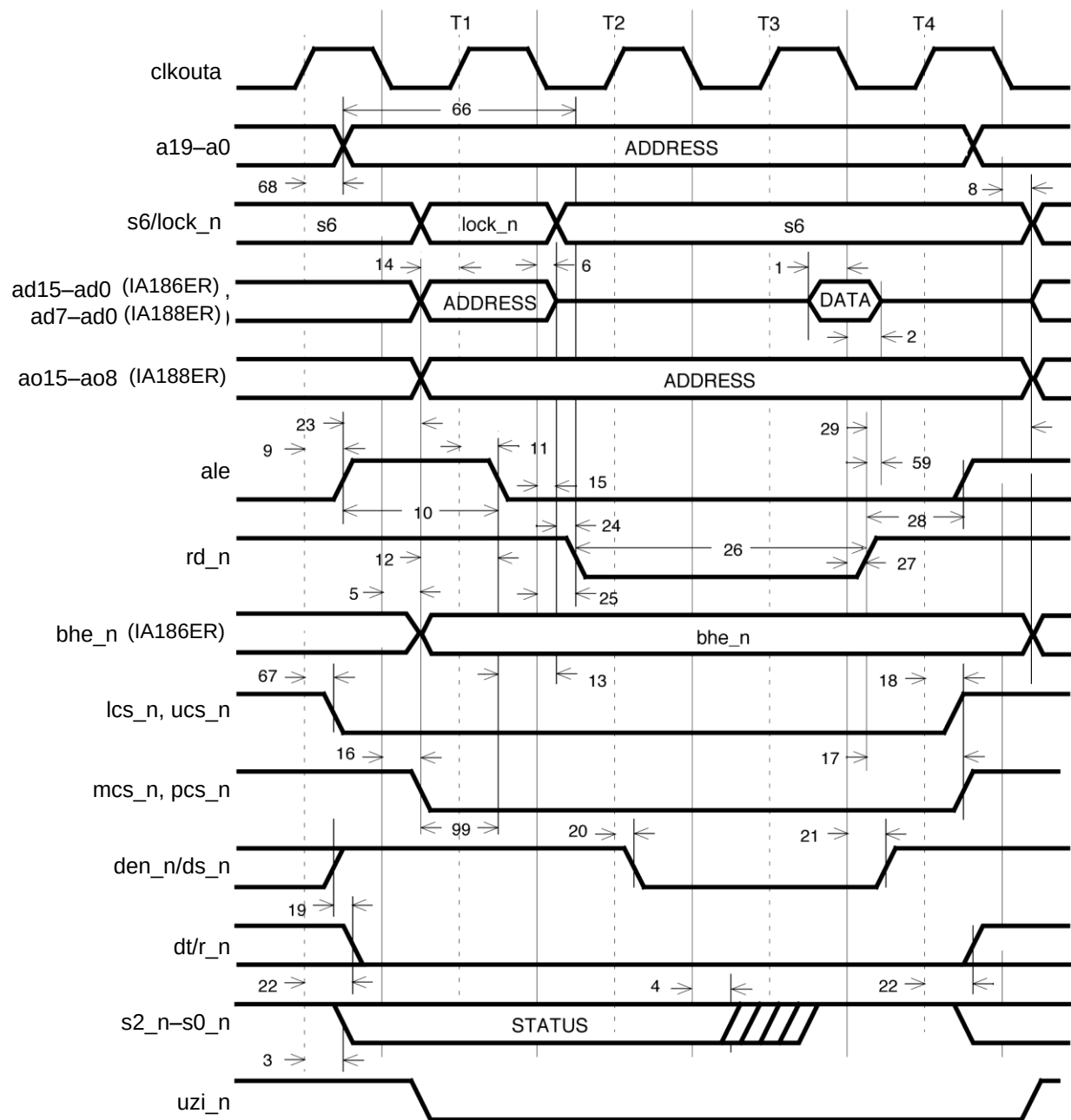
Figure 10. Read Cycle
